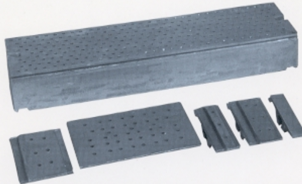
Grates available for the PAD and CAD stokers with improved air hole design. Alloyed gray iron is standard with high silicon/molybdenum ductile iron available for extended service life.
